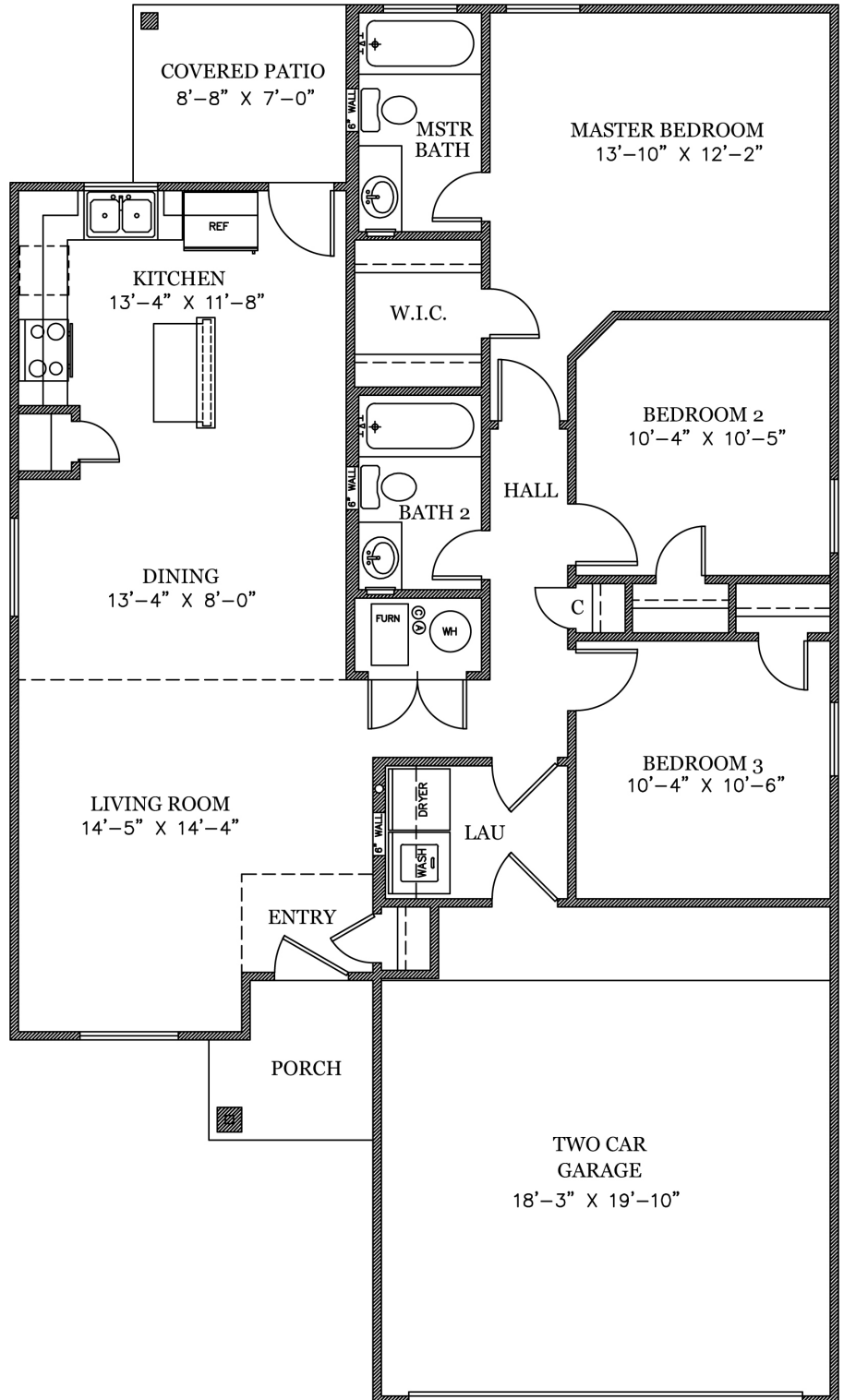
FLOOR PLAN S323
