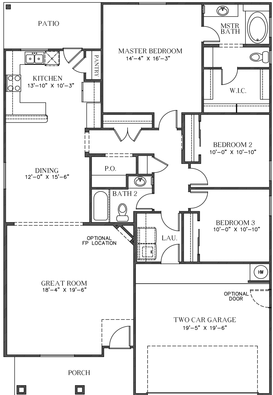
1694 FLOOR PLAN
